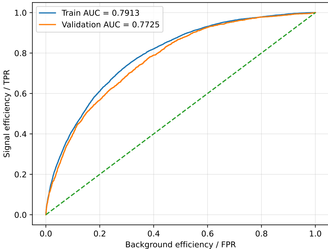
ROC: train vs validation AUC gap = 0.0188
