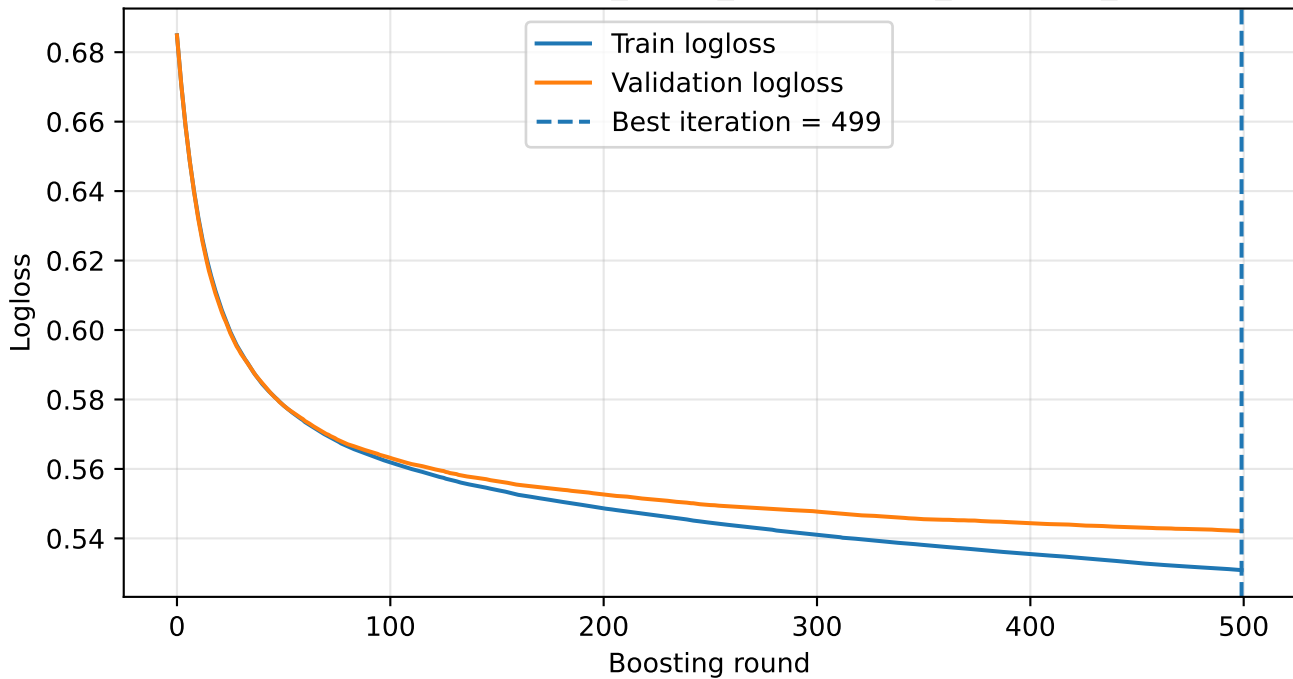
Learning curve: MHc130_MA25_nbkg100000_boost500_none
