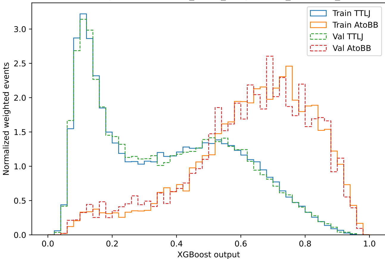
Overtraining check: MHc130_MA25_nbkg100000_boost500_none
