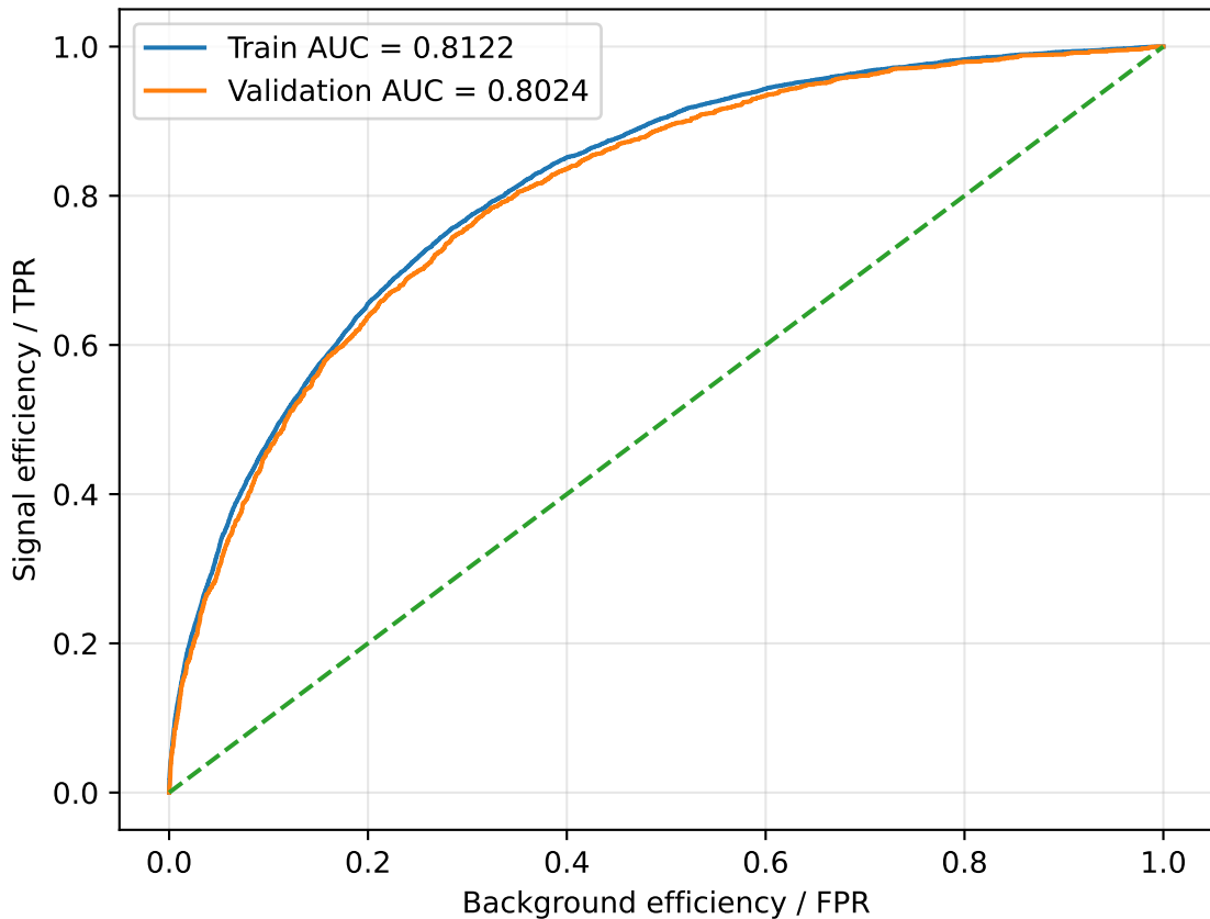
ROC: train vs validation AUC gap = 0.0098
