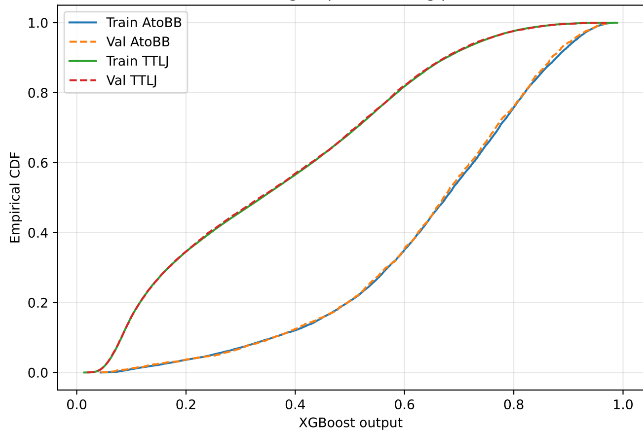
KS check: Signal p=0.621 , Bkg p=0.886
