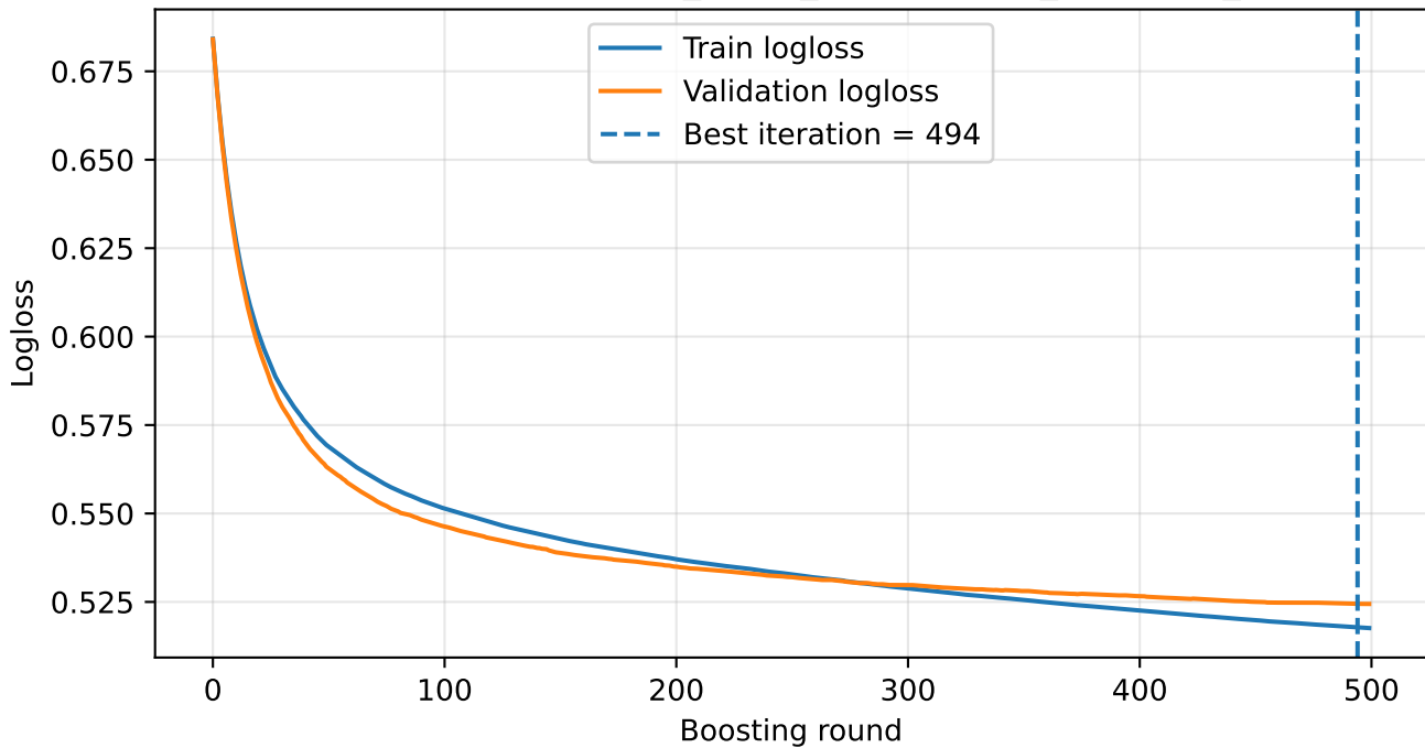
Learning curve: MHc130_MA36_nbkg100000_boost500_none
