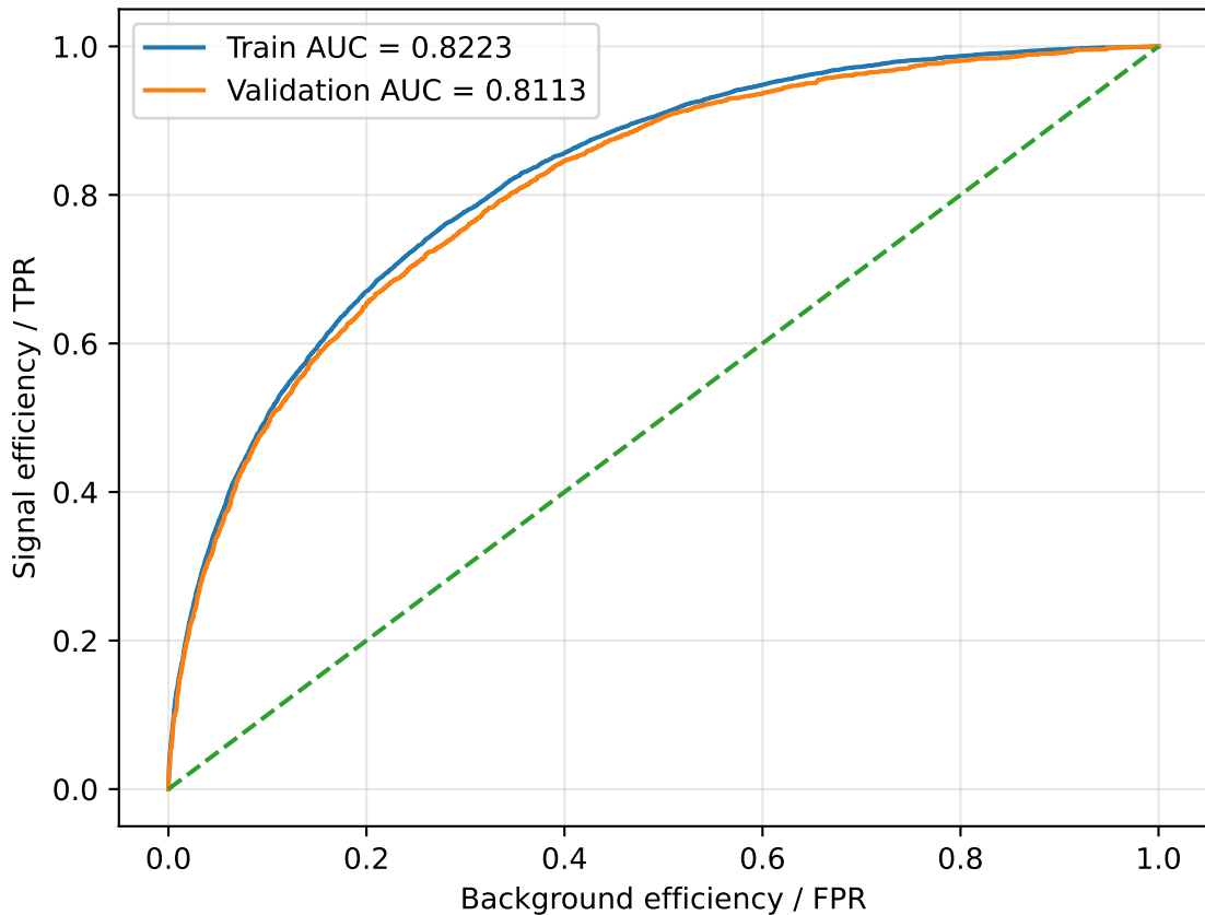
ROC: train vs validation AUC gap = 0.0110
