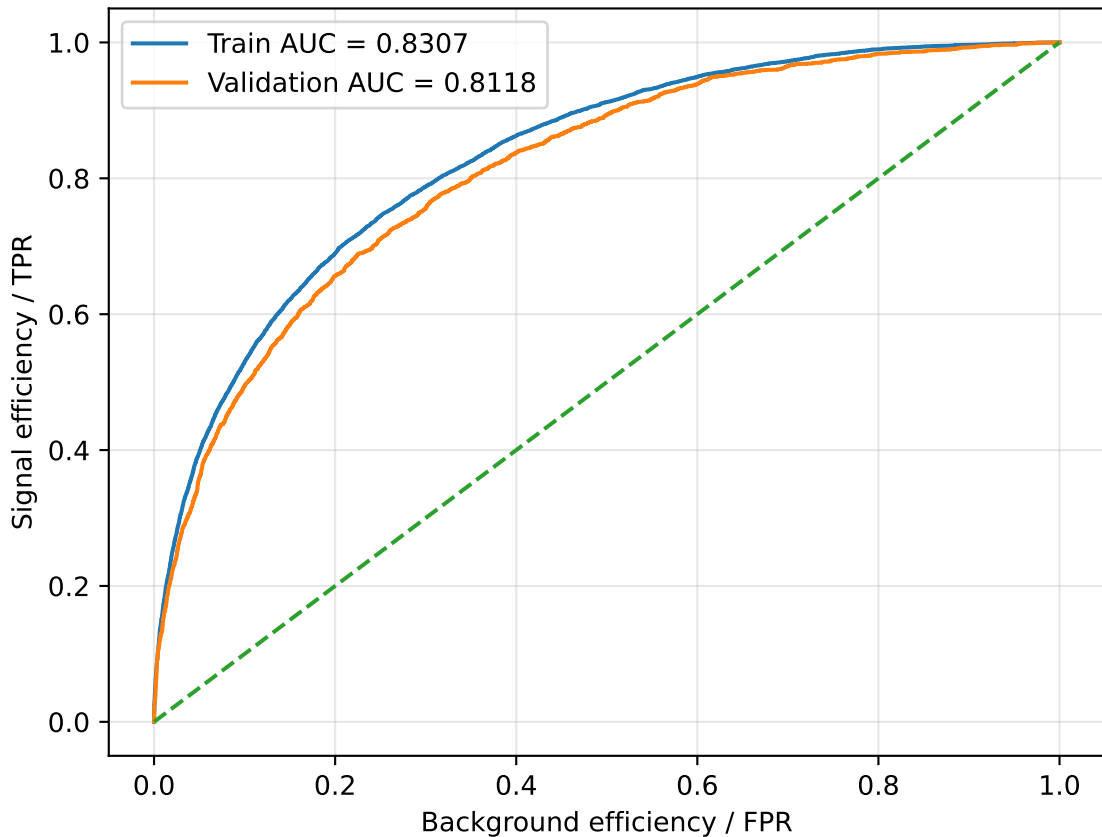
ROC: train vs validation AUC gap = 0.0190
