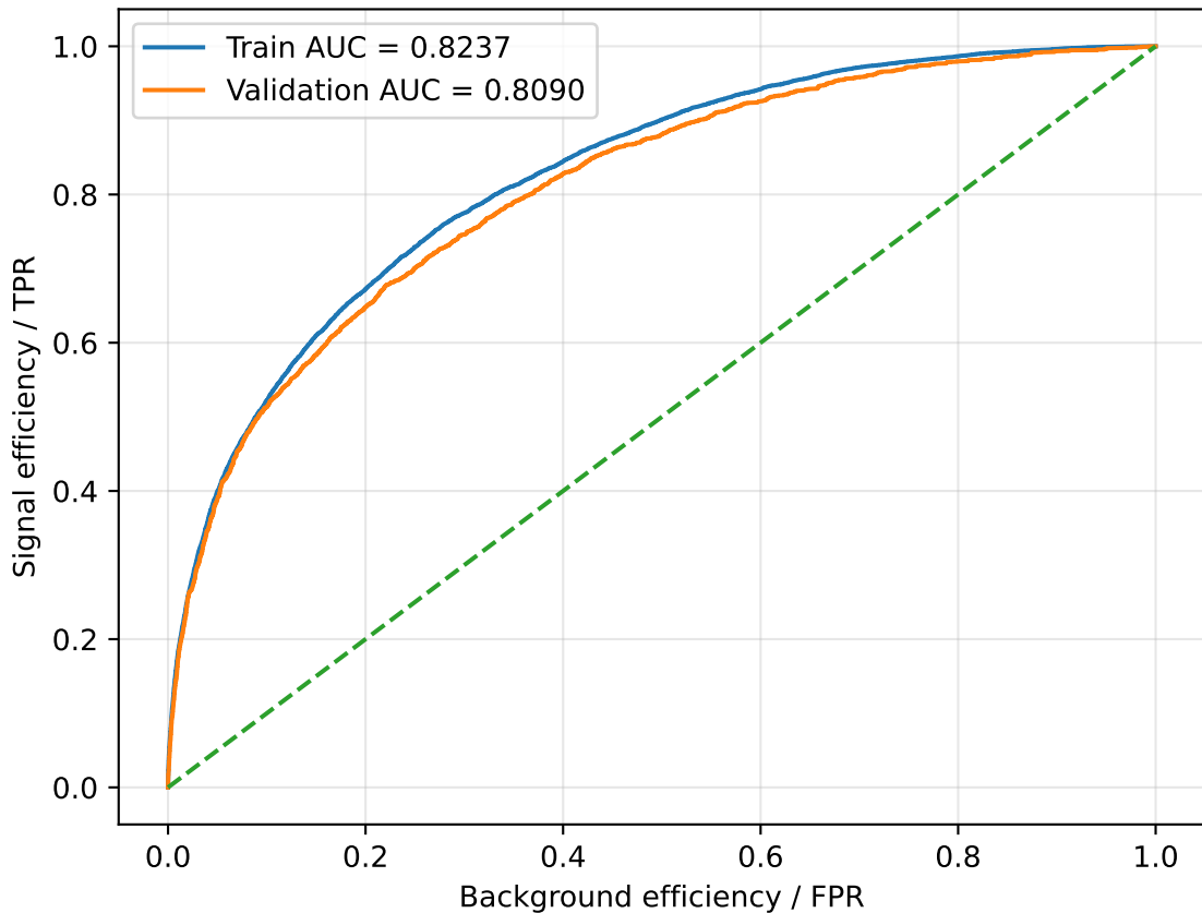
ROC: train vs validation AUC gap = 0.0147
