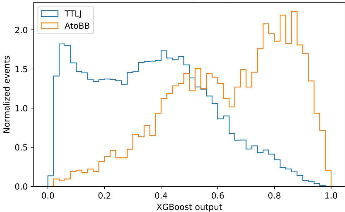
Validation score, shape only: MHc130_MA90_nbkg100000_boost500_none
