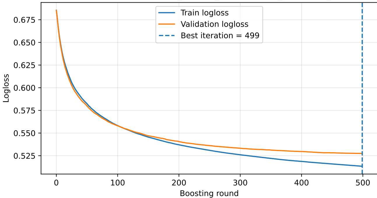
Learning curve: MHc130_MA125_nbkg100000_boost500_none
