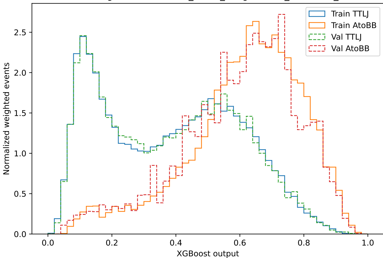
Overtraining check: MHC130_MA18_nbkg100000_boost500_none
