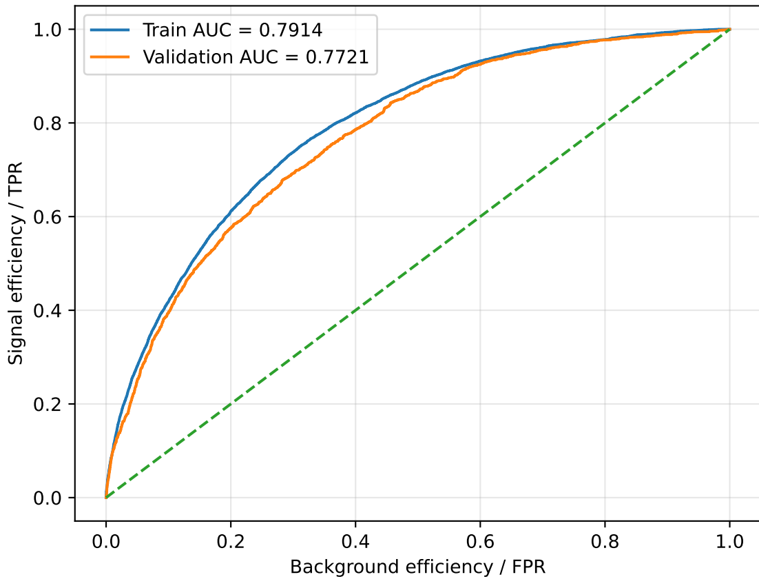
ROC: train vs validation AUC gap = 0.0193
