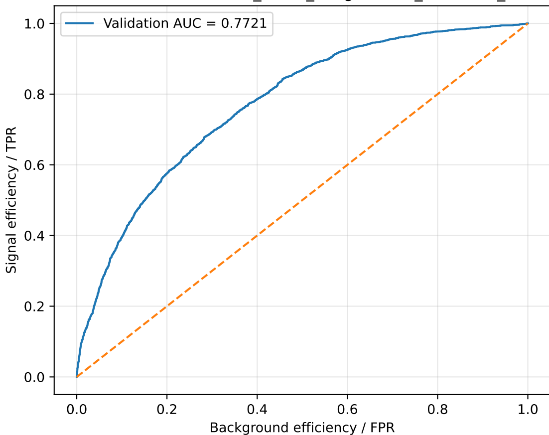
Validation ROC: MHc130_MA18_nbkg100000_boost500_none
