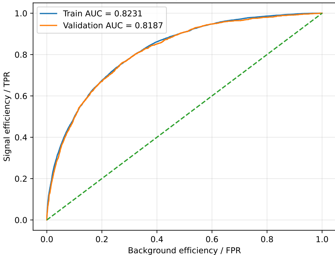
ROC: train vs validation AUC gap = 0.0044
