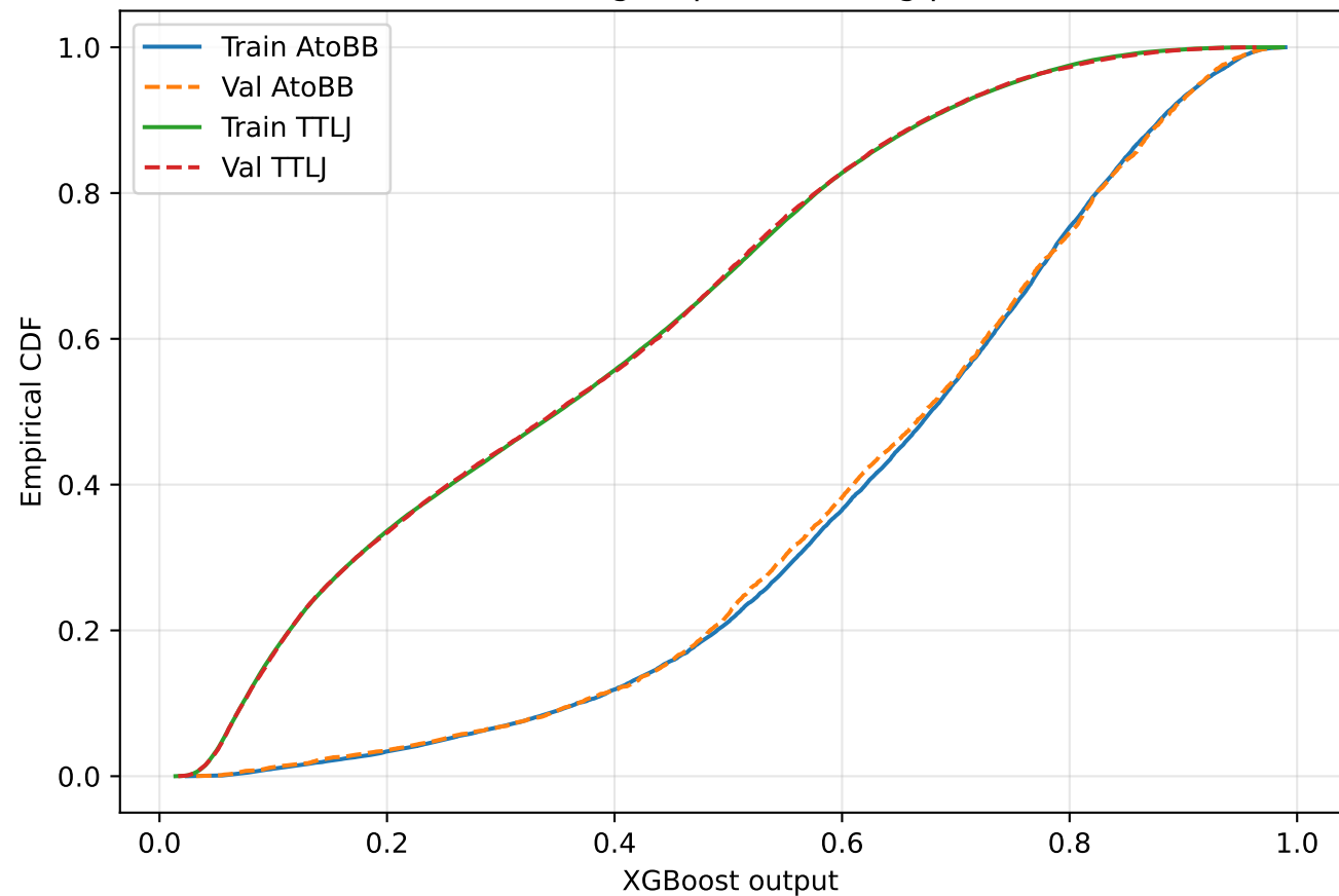
KS check: Signal p=0.172 , Bkg p=0.66
