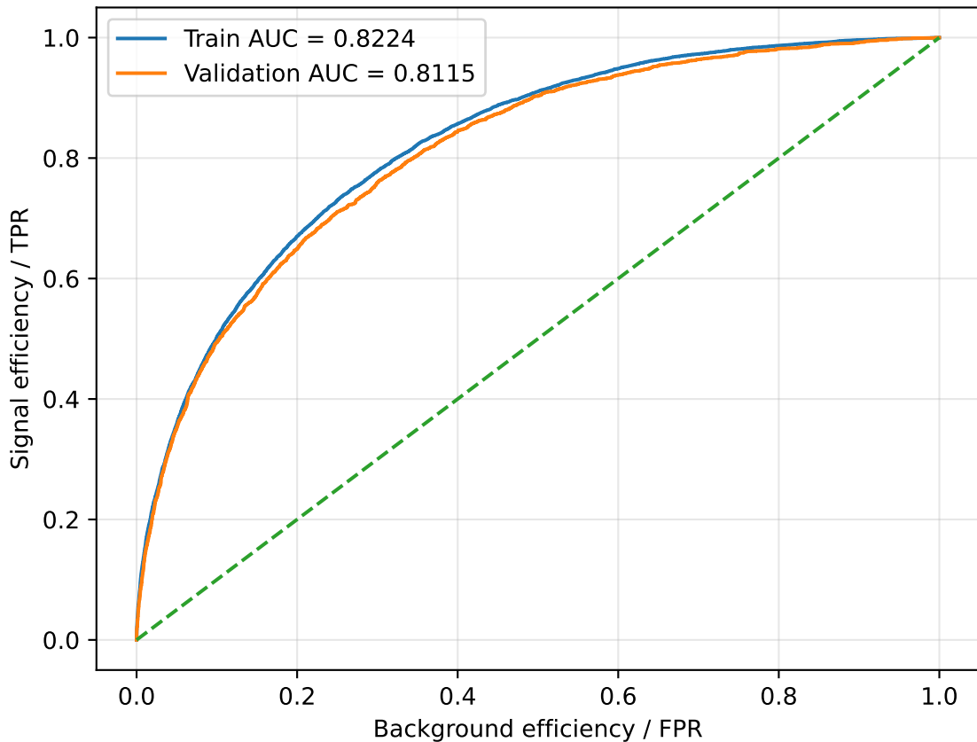
ROC: train vs validation AUC gap = 0.0108
