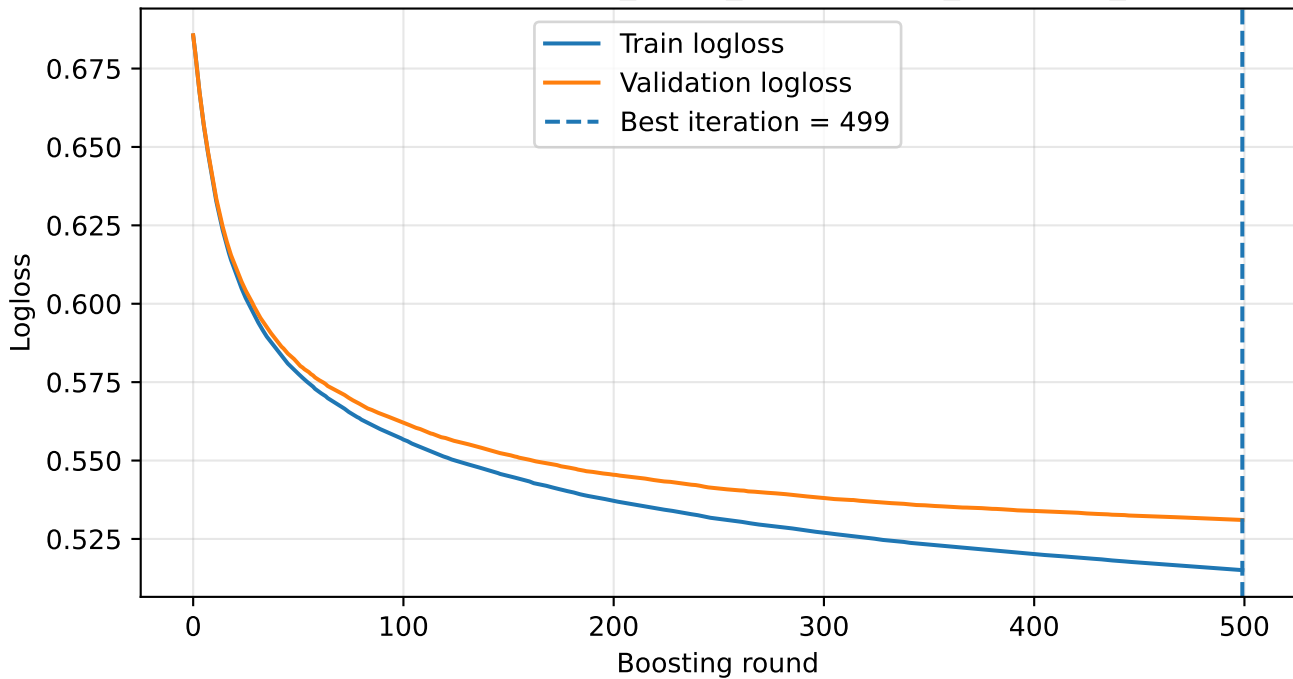
Learning curve: MHc130_MA90_nbkg100000_boost500_none
