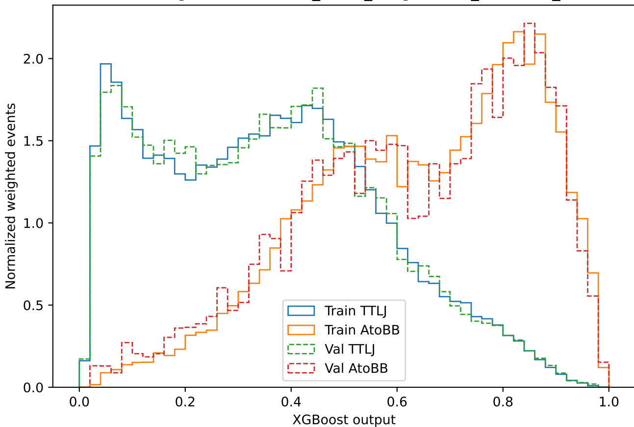
Overtraining check: MHc130_MA90_nbkg100000_boost500_none
