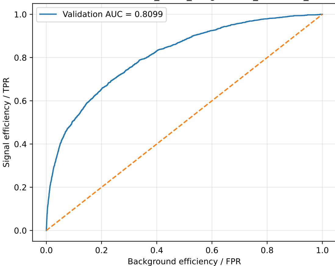
Validation ROC: MHc130_MA90_nbkg100000_boost500_none
