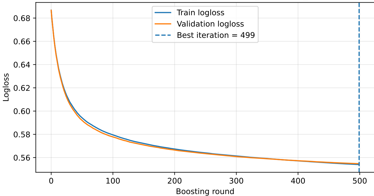
Learning curve: MHc130_nbkg100000_boost500_none
