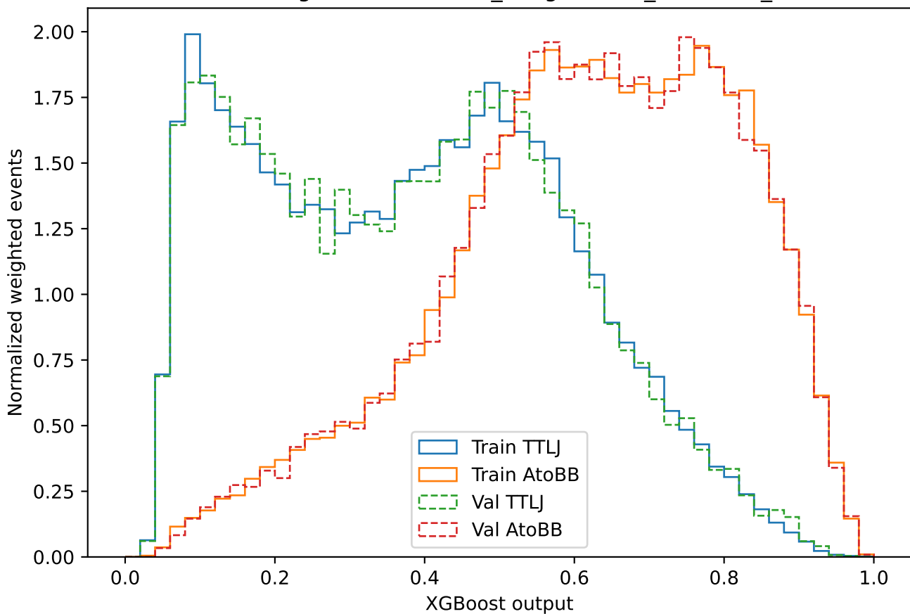
Overtraining check: MHC130_nbkg100000_boost500_none
