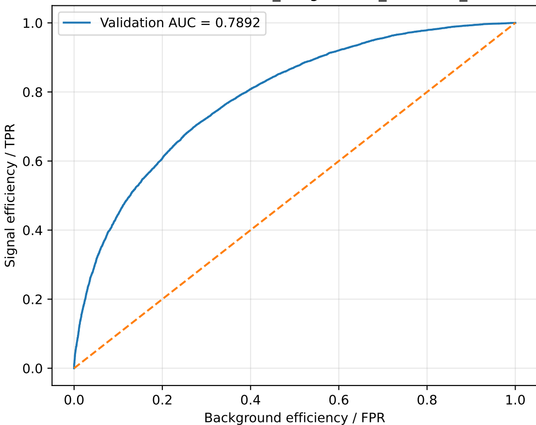
Validation ROC: MHc130_nbkg100000_boost500_none
