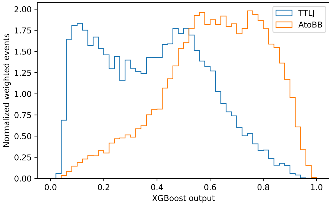
Validation score: MHc130_nbkg100000_boost500_none
