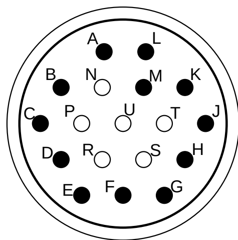
P1 PINOUT, FRONT FACE D38999/26WD18SN INSERT 15-18, KEY N SOCKET CONTACTS
