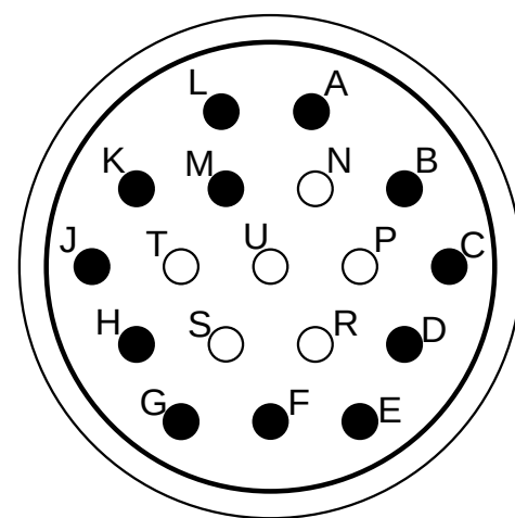
P2 PINOUT, FRONT FACE D38999/26WD18PN INSERT 15-18, KEY N PIN CONTACTS
