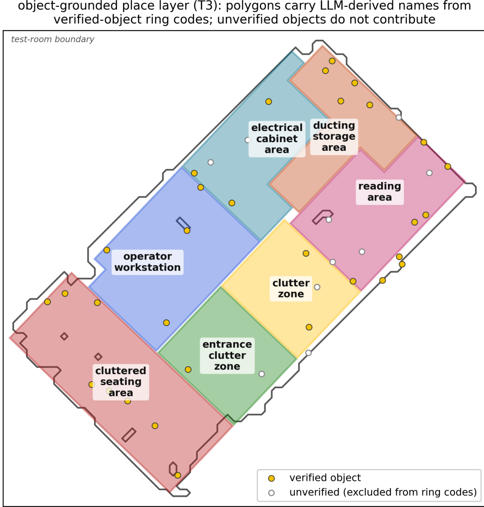
Figure 6: Object-grounded place layer at T3: registered section polygons carry LLM-derived names computed from verified-object ring codes; unverified objects (open markers) do not contribute, so the confidence gate propagates into place semantics.
