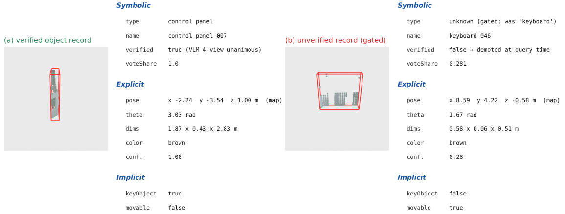
Figure 5: TOSM semantic-object records (symbolic / explicit / implicit layers). (a) A verified record asserts its type. (b) An unverified record is structurally gated at query time: the type is demoted to unknown and the failed classifier guess is quarantined in failedCandidateType .
