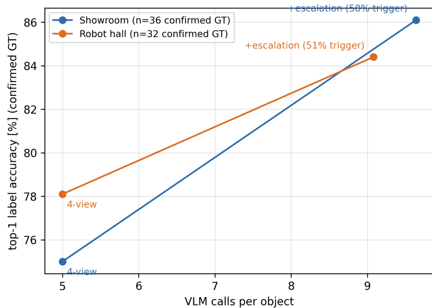
Figure 7. Escalation accuracy–cost curves for both scenes.
