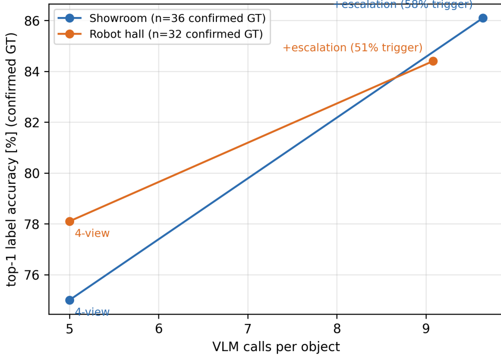
Figure 9: Escalation accuracy–cost curves for both scenes.
