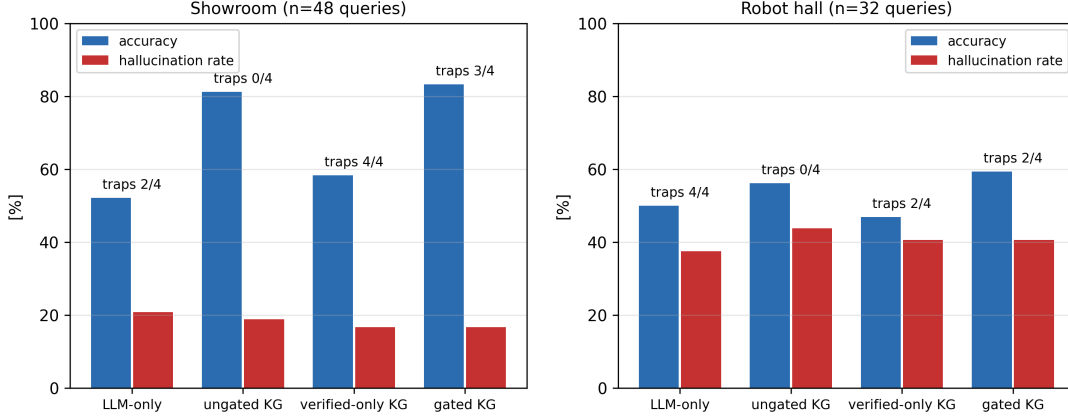
Figure 11: Four-condition query benchmark with trap-question panel.
