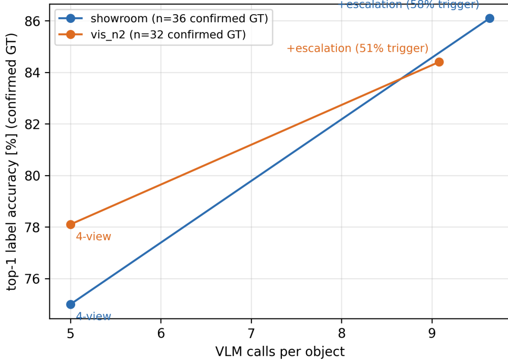
Figure 5: Escalation accuracy-cost curves for both scenes.
