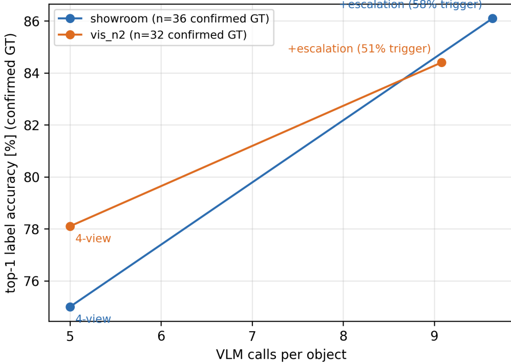
Figure 5: Escalation accuracy–cost curves for both scenes.
