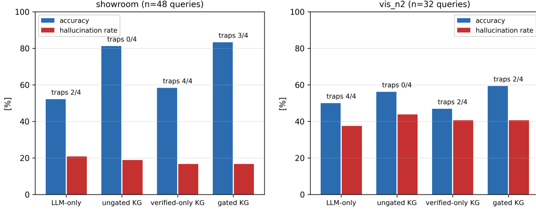
Figure 7: Four-condition query benchmark with trap-question panel.
