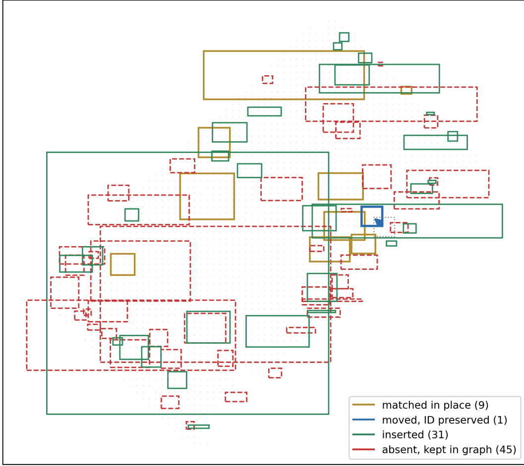
real multi-epoch update of the same room, latest transition (rev 2 \rightarrow 3) (cross-scan registration 4.2-5.1 cm RMSE; identity carried for specific-type objects)
