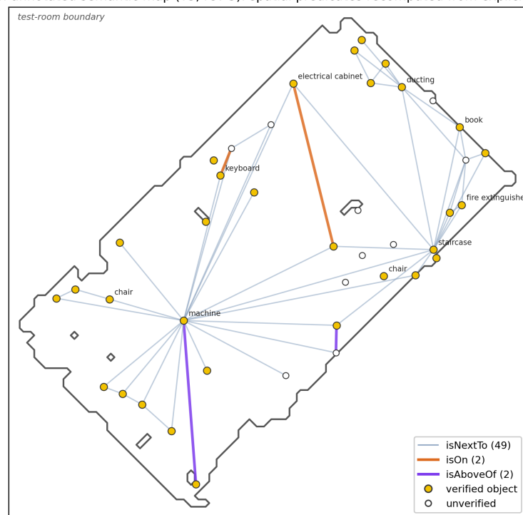
Figure 4. Relation-annotated semantic map (T3): isNextTo , isOn , and isAboveOf edges recomputed from the explicit models at every revision, over verified (filled) and unverified (open) object nodes.
