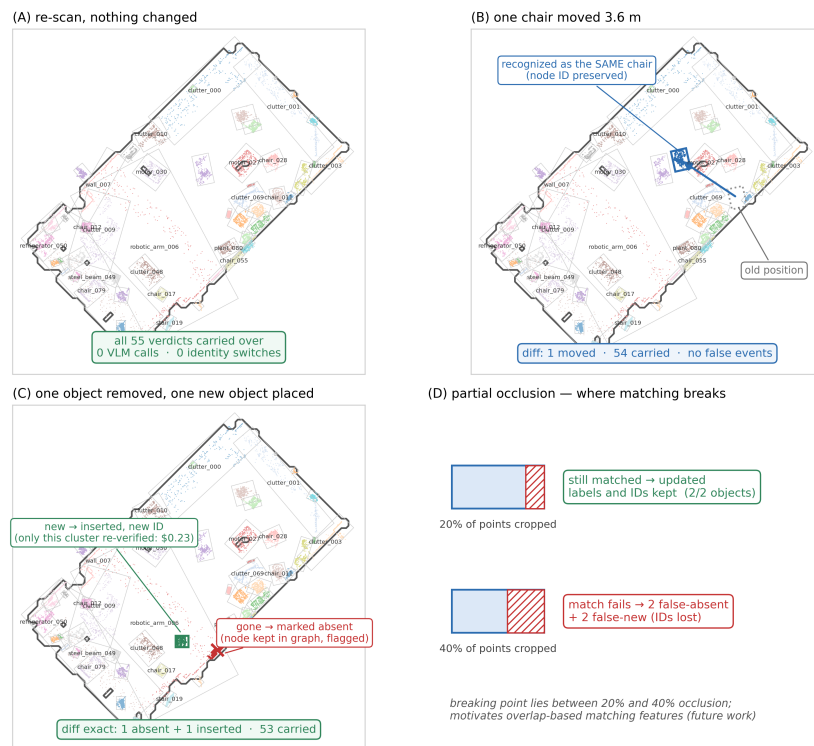
Figure 12. Controlled re-scan scenarios A–D (room-scoped robot hall, 55 objects), top-down view. Colored points are the segmented clusters, thin rotated rectangles their explicit-model footprints with node names, and the dark contour the test-room boundary; each edited object is annotated with the matcher’s decision. (A) A repeat scan with no changes carries all 55 verdicts at zero VLM cost. (B) A 3.6 m chair move is classified moved with its node ID preserved. (C) A removed object is marked absent (node kept and flagged) and a newly placed object is inserted under a new ID; only the insertion is re-verified ($0.23). (D) Partial occlusion: both cropped objects still match at 20%, but at 40% matching fails into two false-absent plus two false-new pairs—the matcher’s quantified breaking point.
