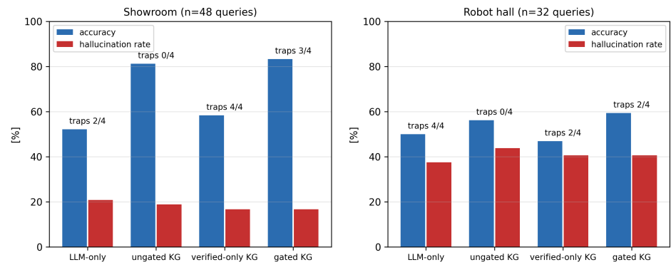
Figure 11. Four-condition query benchmark with trap-question panel.
