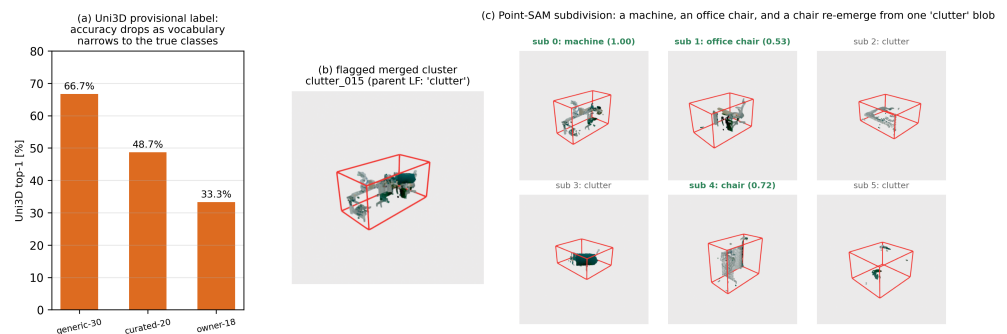
Figure 8. Learned components used as bounded tools. (a) The Uni3D provisional label degrades as the vocabulary narrows to the deployment's true classes (Sec. 5.6)—why it is treated as untrusted context. (b,c) Conditional Point-SAM refinement of a flagged merged cluster: a machine, an office chair, and a chair re-emerge from a single clutter blob, each re-verified independently.
