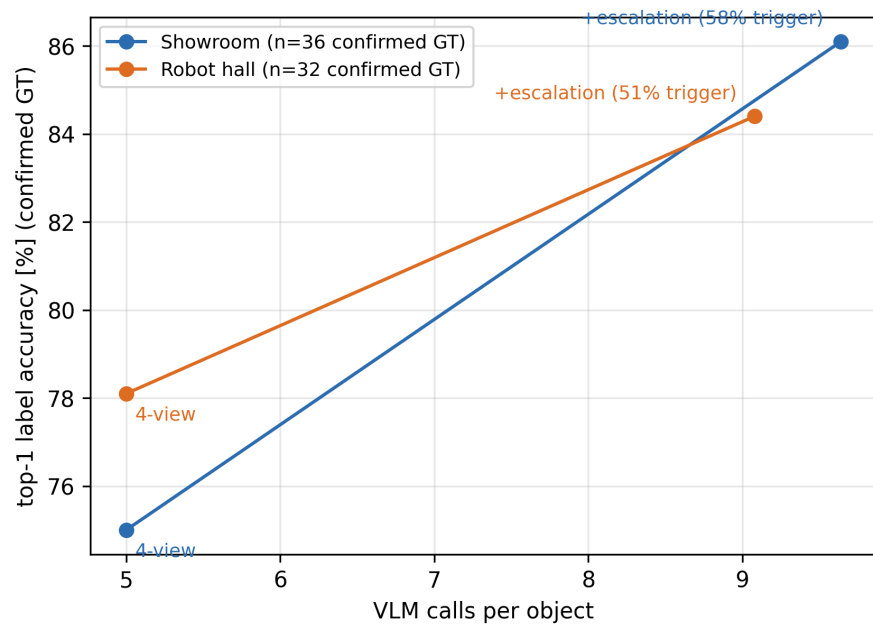
Figure 9. Escalation accuracy–cost curves for both scenes.
