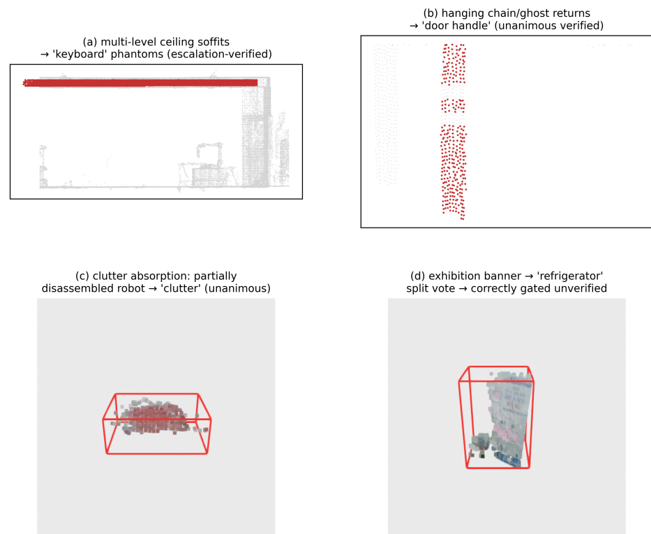
Figure 10. Verification error taxonomy: remnant phantom, unanimous-but-wrong, clutter absorption, render ambiguity.
