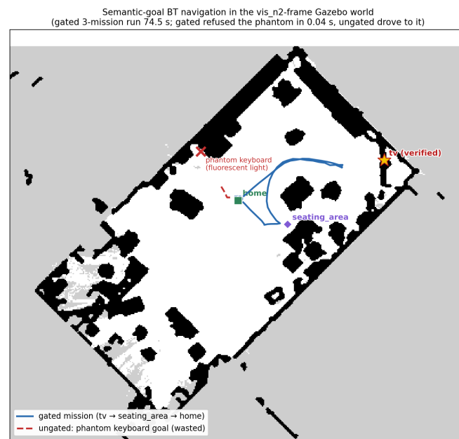
Figure 16. Semantic-goal navigation in the Gazebo twin of the test room (world, map, and knowledge graph share the exploration-scan frame). Blue: a gated three-mission run (TV → seating area → home). Red dashed: an ungated run drives to a phantom keyboard — a fluorescent lamp that verification refuses under the gated view.
