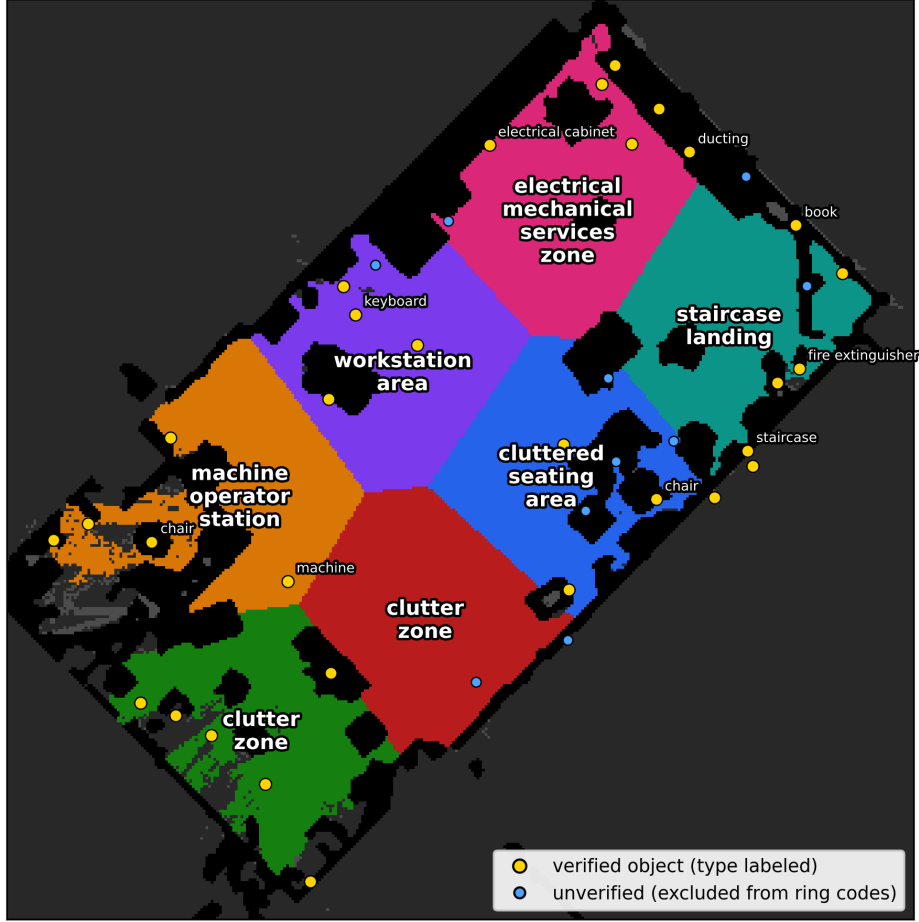
object-grounded place layer (T3): SLIC superpixel regions over the nav-stack grid map; LLM-derived names from verified-object ring codes (black = obstacles)
