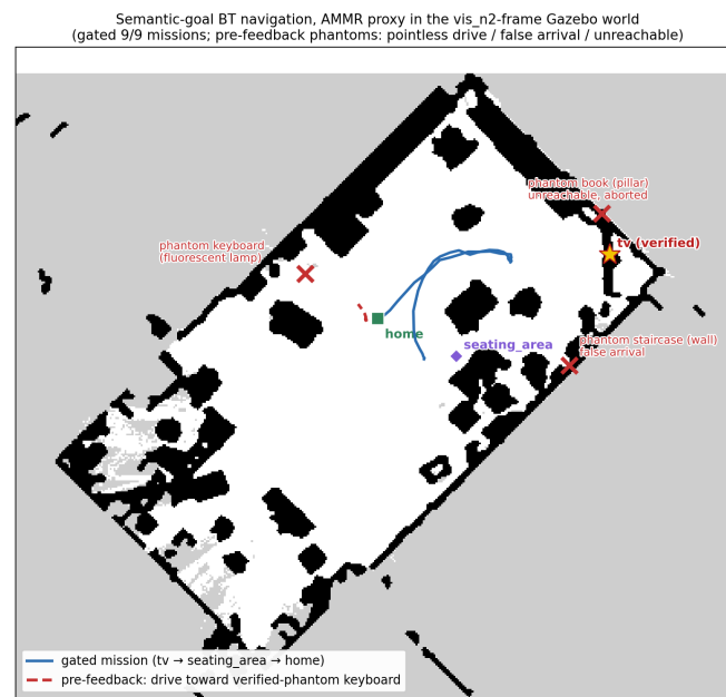
Figure 16. Semantic-goal navigation of the AMMR proxy in the Gazebo twin of the test room (world, map, and knowledge graph share the exploration-scan frame). Blue: a gated three-mission run (TV → seating area → home). Red dashed: against the pre-feedback graph the robot drives toward a verified-phantom keyboard — a fluorescent lamp; crosses mark the three phantom goals with their failure modes (pointless drive, false arrival, unreachable). All three are refused once structure filtering and owner feedback are applied.
