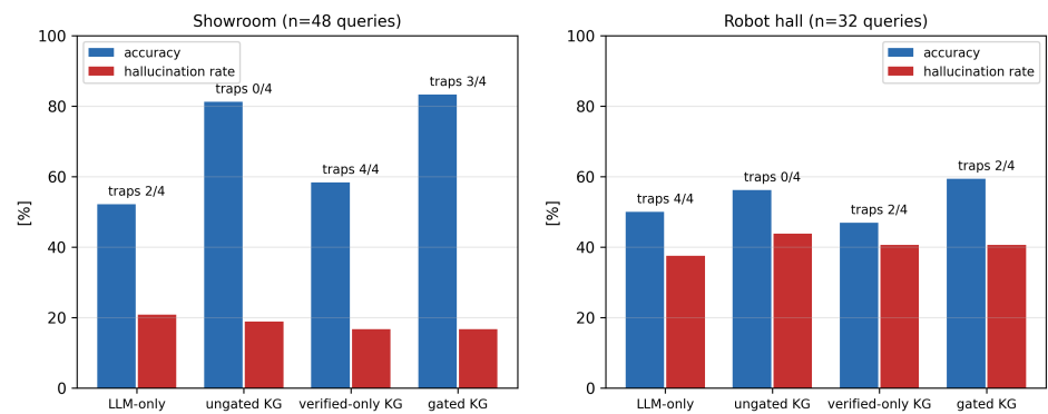
Figure 12. Four-condition query benchmark with trap-question panel.
