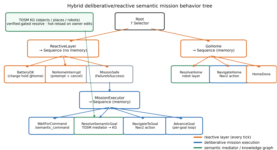
Figure 15. Hybrid deliberative/reactive mission behavior tree. The reactive layer re-evaluates battery and interrupt conditions every tick and can preempt navigation (canceling the active Nav2 goal); the deliberative branch resolves semantic commands through the TOSM mediator, which hot-reloads the knowledge graph when the management console edits it.
