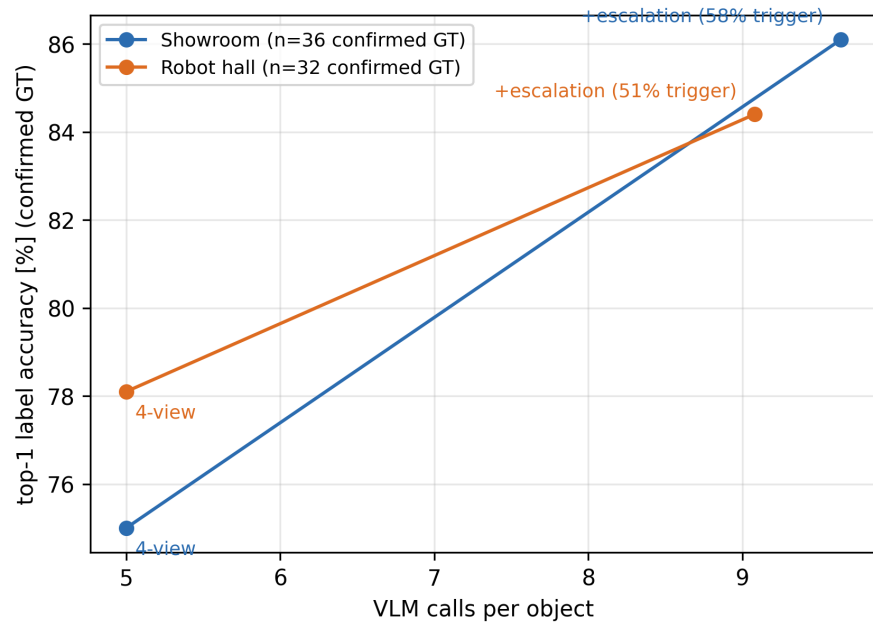
Figure 10. Escalation accuracy–cost curves for both scenes.
