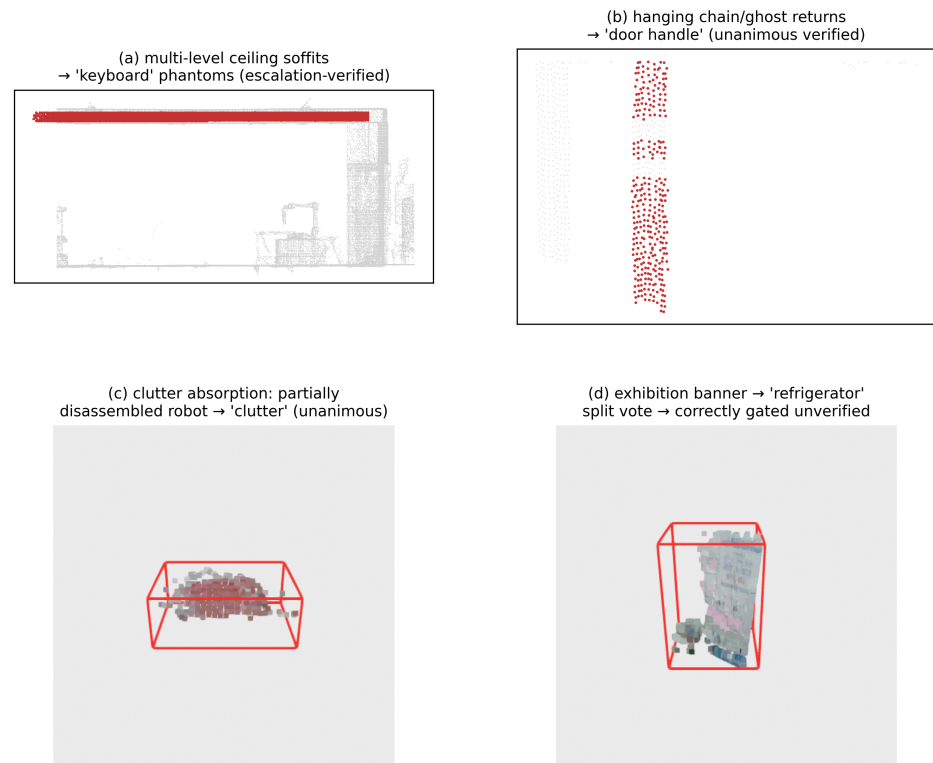
Figure 11. Verification error taxonomy: remnant phantom, unanimous-but-wrong, clutter absorption, render ambiguity.
