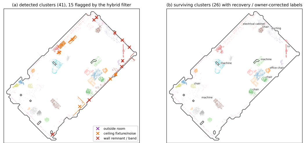
Figure 9. Hybrid structure-noise filter on the T3 epoch. (a) All 41 detected clusters; the 15 flagged ones are colored by rule — wall remnant/band (grid-map hug \times thin vertical sheet, or long full-height band), ceiling fixture/noise, outside the room boundary. (b) The 26 survivors with recovery / owner-corrected labels. The wall-flush monitor bank (labeled tv ) and wall-mounted equipment survive; residual merge labels ( electrical cabinet , ducting ) are retained pipeline output, not corrections.
