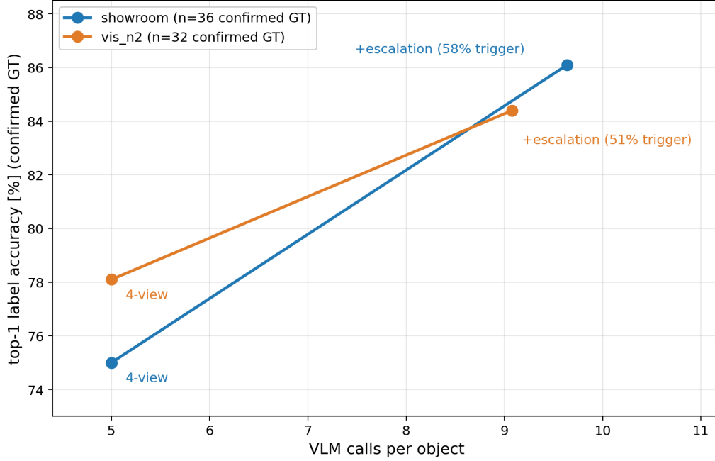
Figure 5: Escalation accuracy–cost curves for both scenes.
