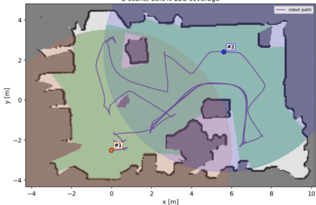
Run 2 (run4) -- Isotropic disk: 2 scans, 85.5% LOS coverage
