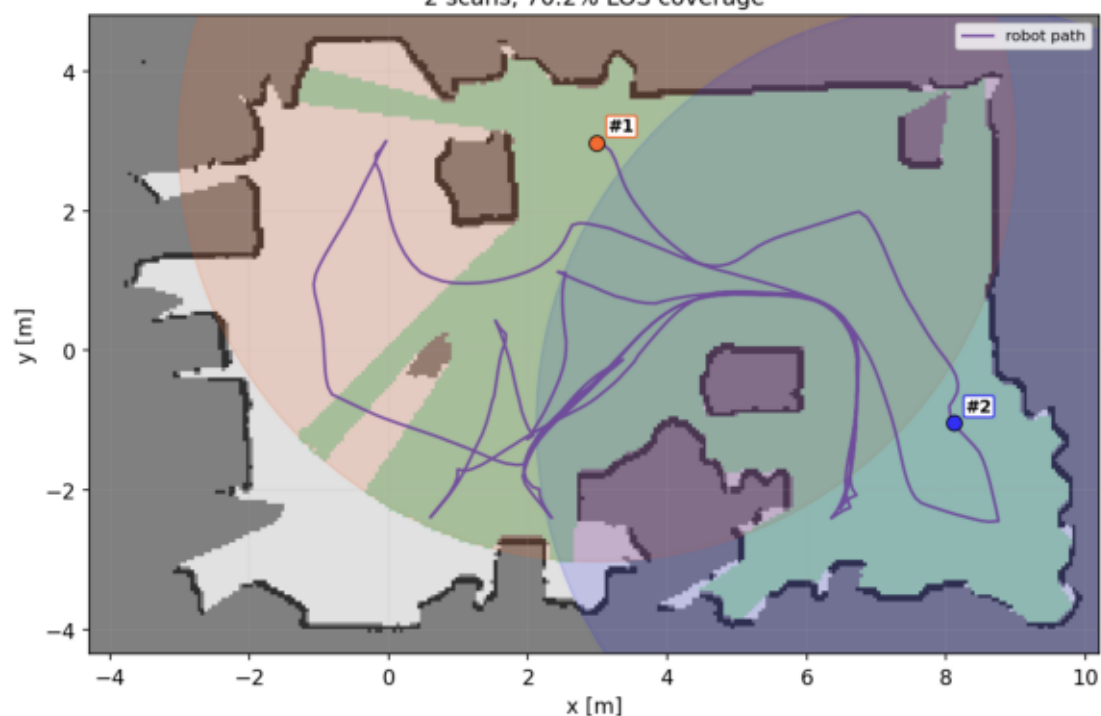
Run 3 (run5) -- Isotropic disk: 2 scans, 70.2% LOS coverage
