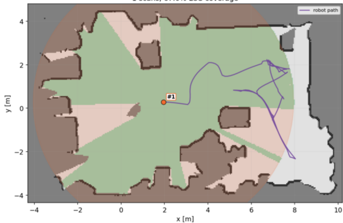
Run 1 (run1) -- Isotropic disk: 1 scans, 67.0% LOS coverage
