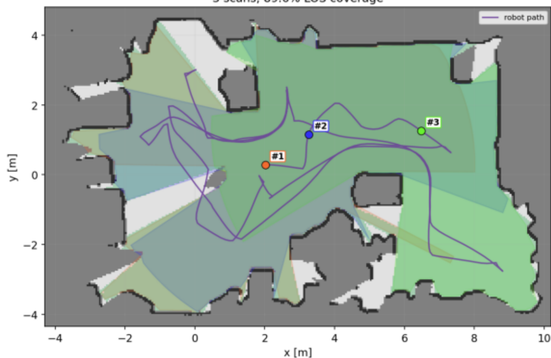
Run 4 (gz2) -- Ray-cast visibility (proposed): 3 scans, 89.6% LOS coverage
