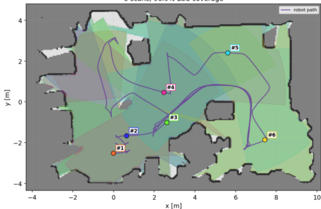
Run 2 (run4) -- Ray-cast visibility (proposed): 6 scans, 96.9% LOS coverage
