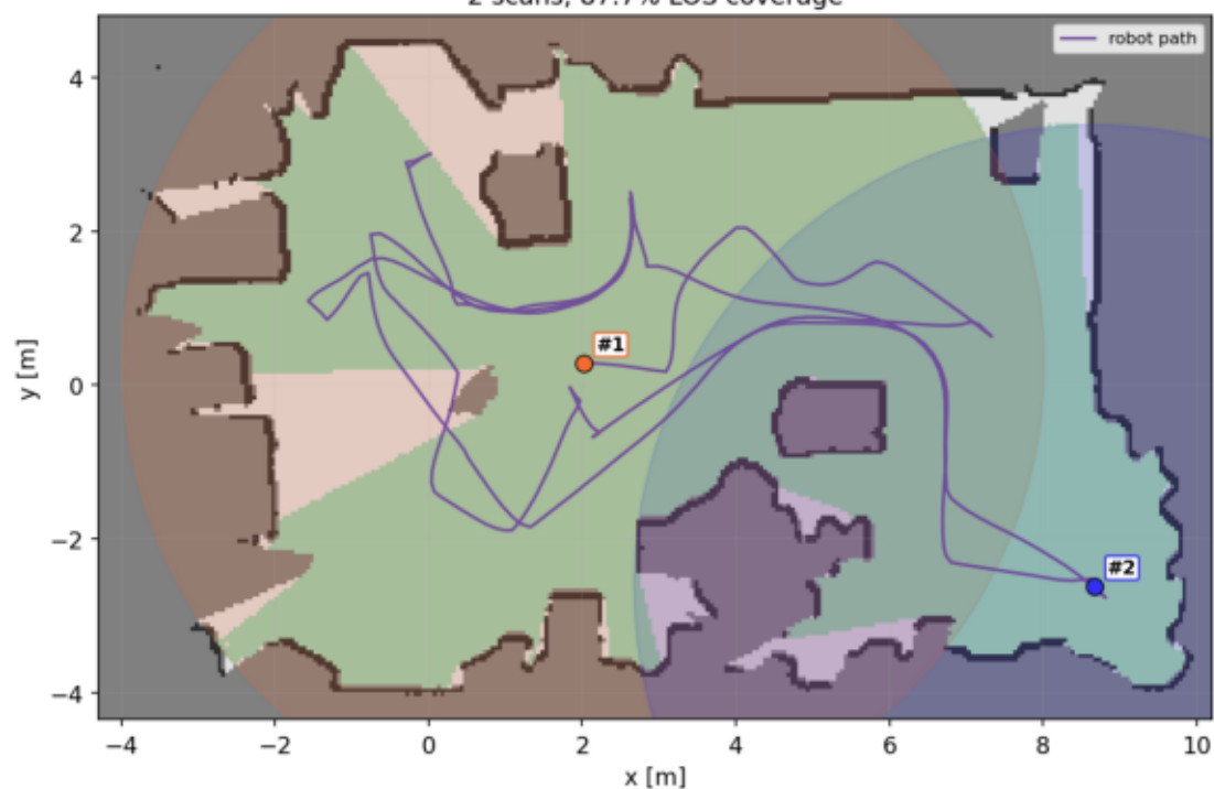
Run 4 (gz2) -- Isotropic disk: 2 scans, 87.7% LOS coverage
