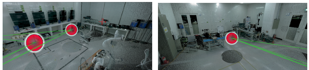
Figure 15. Interior views of the registered colorized point cloud of visibility run 3, rendered along two diagonal viewing directions: (Left) Toward the display wall with its monitor and product-panel arrays; (Right) Toward and toward the equipment and workbench side of the room (right) . Red markers and green edges are the scan stations and cloud-to-cloud links of Table 4; the five autonomously acquired scans fuse into a single coherent survey-grade model of the room.
