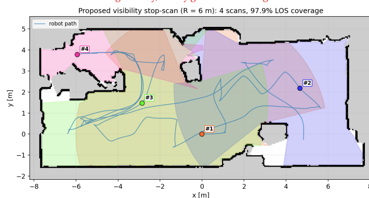
Figure 5. Proposed visibility stop-and-scan on the single-room world ( R = 6 m): 4 scans, 97.9% LOS coverage. The map, robot path, Each accepted scan pose (marker) and per-scan its visibility polygons (polygon share one color, indexed by scan order (#1...#4) are overlaid on; the Cartographer grayscale background is the occupancy map (light gray free, black occupied, darker gray unknown) and the blue line is the robot path. The same color convention is used in all placement figures.
