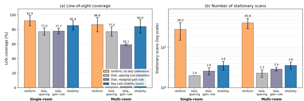
Figure 8. Three-way Four-way skip-rule comparison on identical paths ( N = 5 single-room and N = 10 multi-room trajectories, paired per path) – uniform no-skip reference, isotropic-disk baseline, and ray-cast visibility (ours). (a) LOS coverage; (b) stationary scan count on a , log scale (mean \pm s.d.). The visibility rule improves LOS over the disk baseline (single-room 77.0 \rightarrow 85.4%; multi-room 77.0 \rightarrow 84.0%) while using only a small fraction of the uniform reference's scan count (28.0/40.8 scans);
