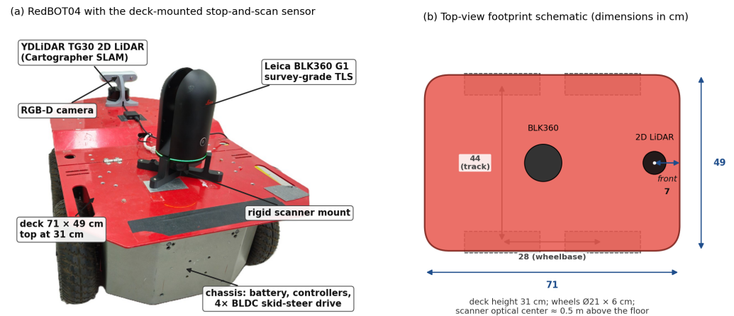
Figure 3. RedBOT04, the four-wheeled mobile scan platform used for. (a) Annotated view with the real-hardware experiments, carrying a deck-mounted Leica BLK360 G1 terrestrial laser scanner; (black unit, center b) as its survey-grade stationary sensor top-view footprint schematic with the principal dimensions (cm). The platform additionally carries a 2D LiDAR and an RGB-D camera for Cartographer SLAM and Nav2 navigation.
