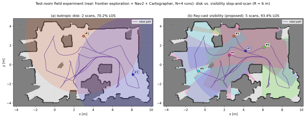
Figure 13. Fully autonomous on-hardware disk-versus-visibility comparison in the physical test room (RedBOT04 running frontier exploration + Nav2 + Cartographer live; representative of N = 4 completed runs), stop-and-scan at; R = 6 m). Light grey is: mapped free space; dark grey is: unmapped; black is: occupied; the purple line is the: autonomous robot path and; colored markers are the: placed scans with their coverage regions. (a) The disk model places few scans and leaves the occluded bays uncovered Disk spacing rule; (b) the visibility model scans them rule.
