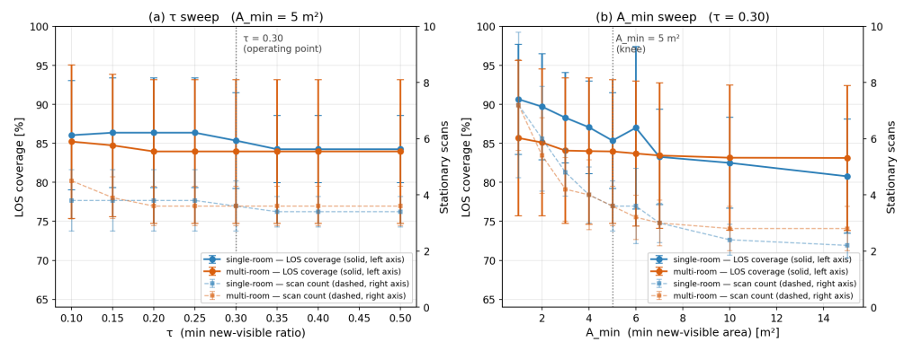
Figure 11. Parameter sweep (by deterministic replay on the fixed candidate paths (mean \pm s.d. over N = 5 single-room and N = 10 multi-room paths)). Solid curves: LOS coverage (left axis); dashed curves: scan count (right axis). (a) \tau sweep at A_{\min} = 5 \text{ m}^2 : coverage and scan count are flat across \tau \in [0.10, 0.50] ; (b) A_{\min} sweep at \tau = 0.30 : A_{\min} is the operative coverage-vs-scans knob, with the knee at 5 \text{ m}^2 marked.
