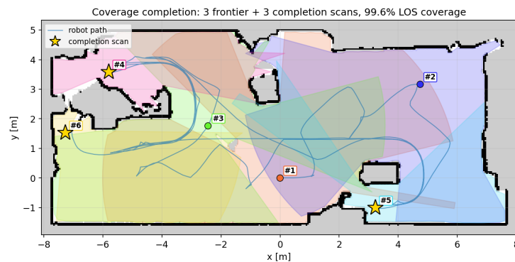
Figure 10. Coverage completion. After frontier exploration, the robot drives into each still-uncovered pocket and scans (*) until none above the minimum pocket area remains. Here 3 frontier + 3 completion scans, 99.6% LOS.
