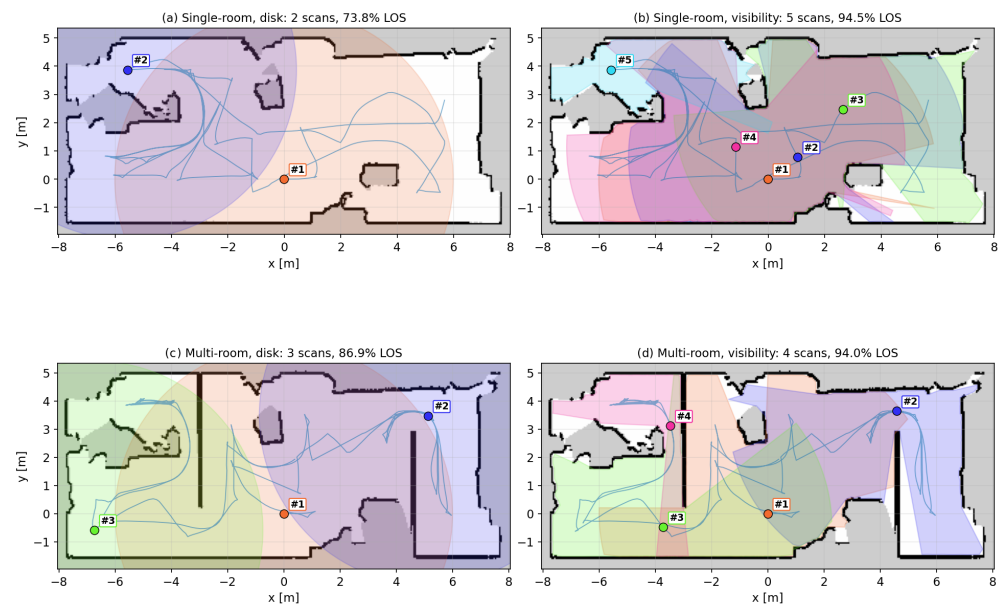
Figure 7. Controlled skip-rule ablation on an identical map and identical candidate path; only the skip decision differs. (a,b) single-room Single-room and (c,d) multi-room, each multi-room, each under the disk spacing rule (a,c) and the visibility rule (b,d) . The disk rule is structurally capped at 2–3 scans and leaves occluded pockets/rooms ( \approx 74\text{--}87\% LOS); the visibility rule fills them ( 94\text{--}95\% LOS).
