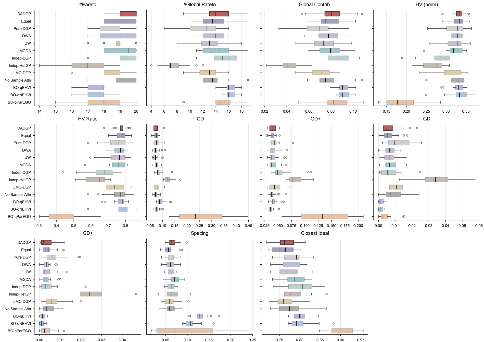
Per-run robust Pareto indicator distributions across 20 MOO runs
