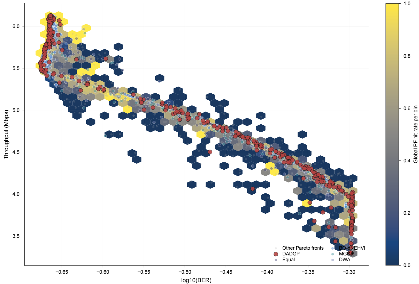
BER-throughput attainment with DADGP highlighted
