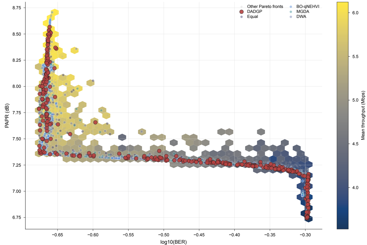
BER-PAPR projection with throughput field
