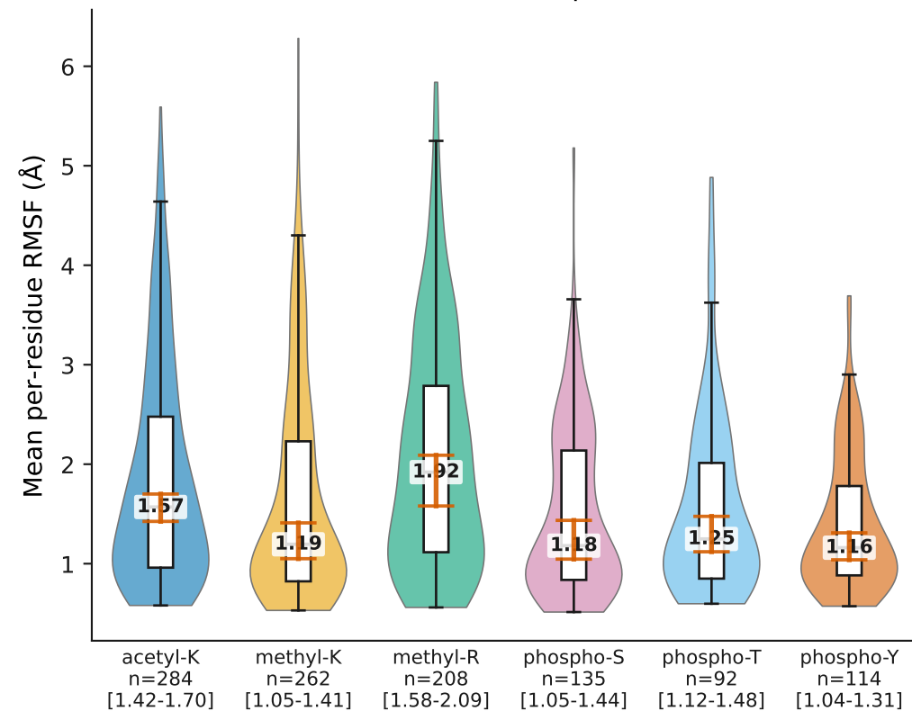
C. Per-residue RMSF (mean across protein)
