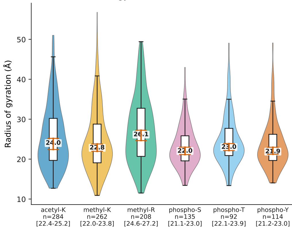
B. Protein radius of gyration
