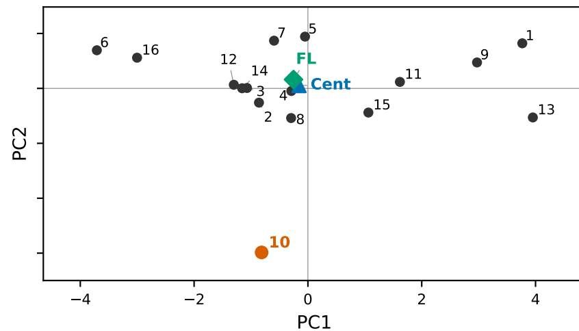
Elastic Net
