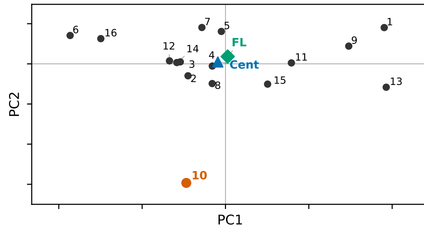
Elastic Net
