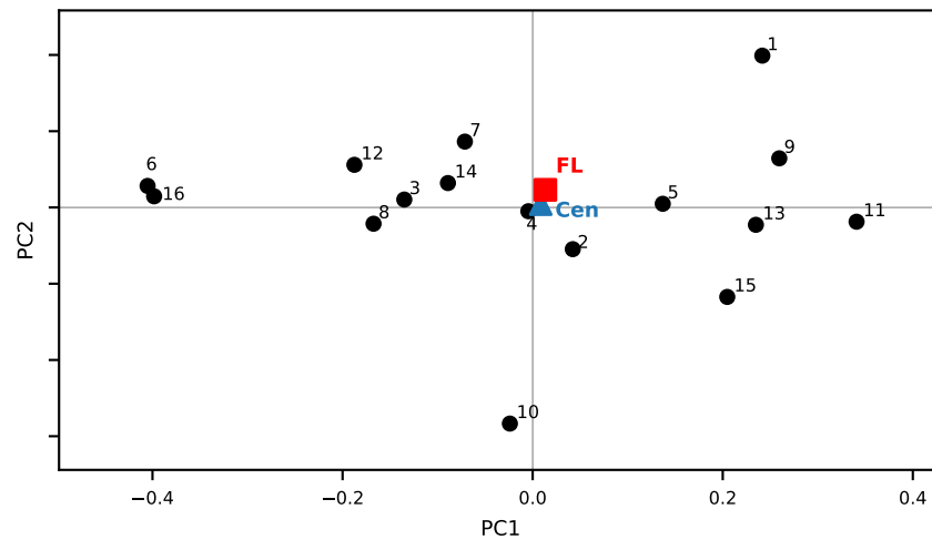
Elastic Net
