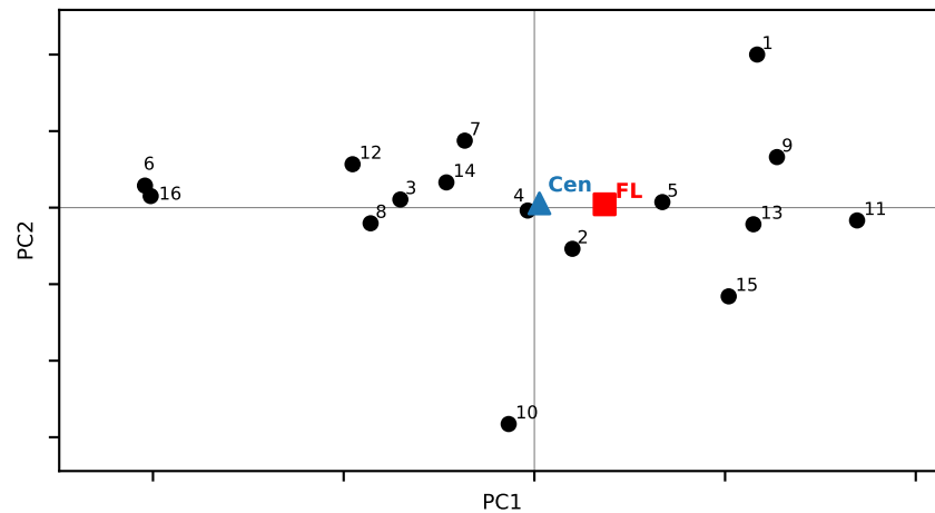
Elastic Net
