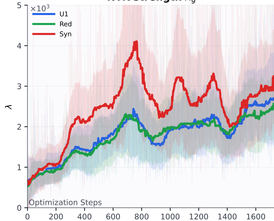
NTK strength \lambda_g
