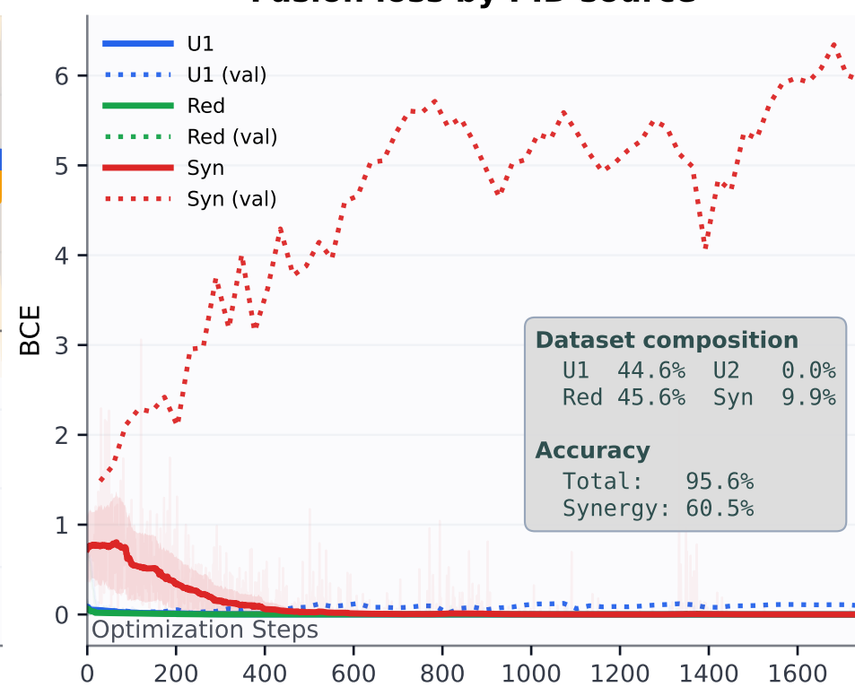
Fusion loss by PID source
