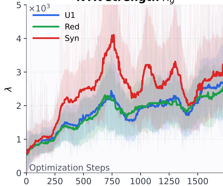
NTK strength \lambda_g
