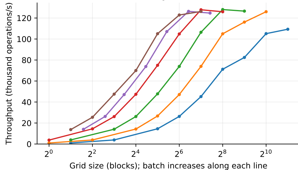
KeyGen
