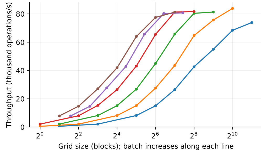
Decaps
