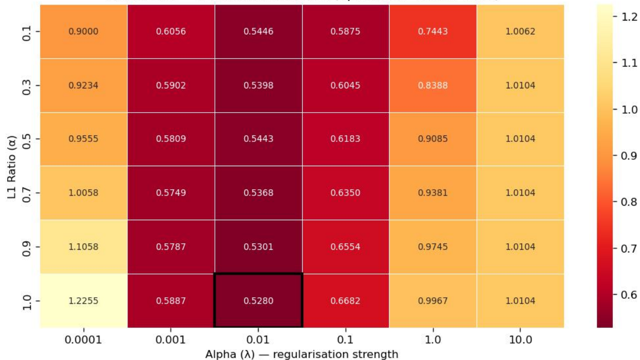
Elastic Net — 5-fold CV RMSE Grid (optimal: \alpha=1.0 , \lambda=0.01 )
