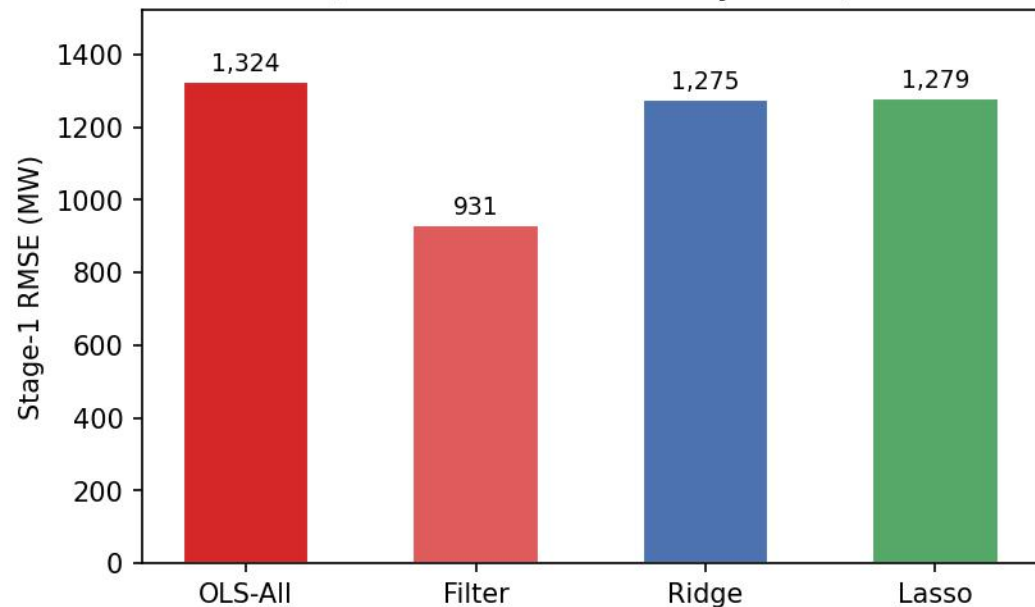
Stage-1 RMSE per Strategy (OLS-All: multicollinearity effect)
