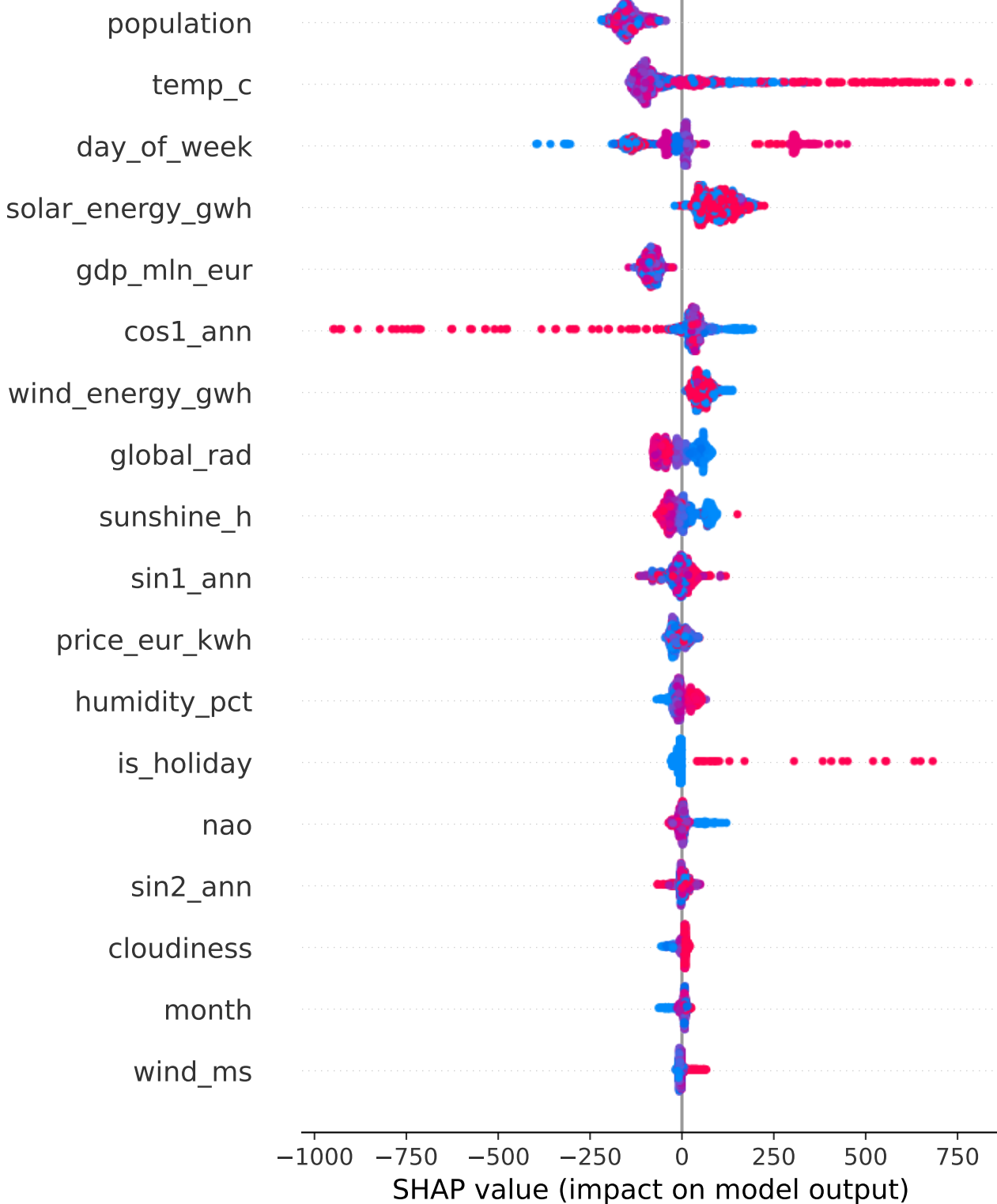
SHAP Beeswarm — Strategy 0: OLS-All (unregularised)
