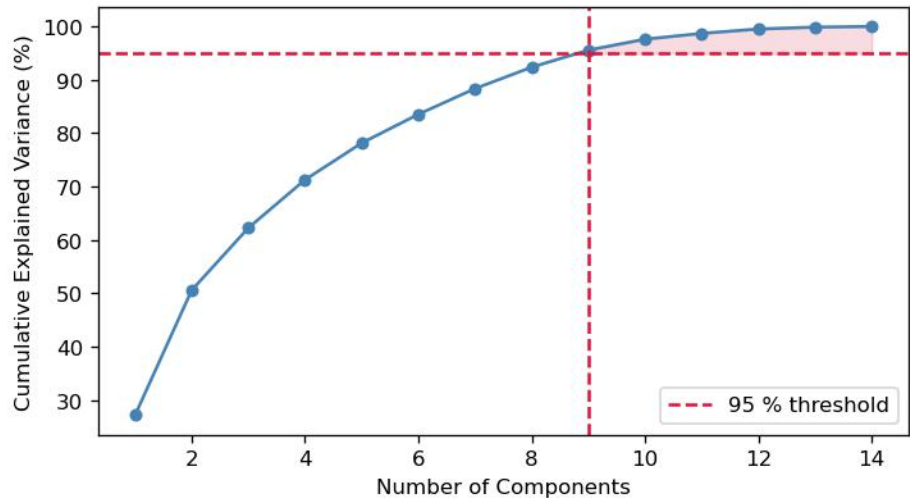
Cumulative Variance
